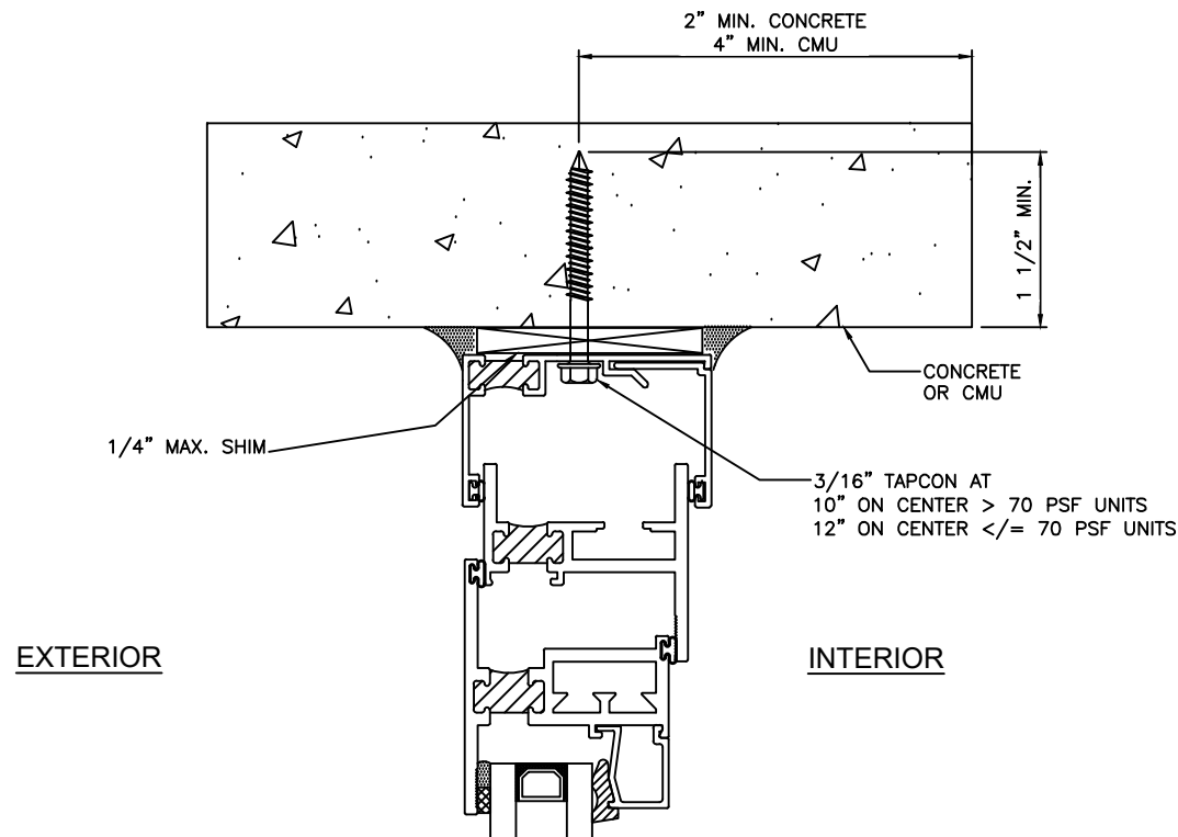
SECTION 1/1, 1/2 & 1/3 RECEPTOR TO CONCRETE OR CMU SUBSILL SIMILAR
