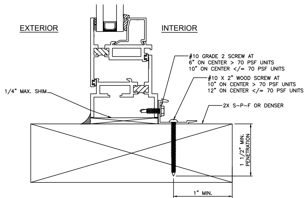
SECTION 1/1, 1/2 & 1/3 INSIDE CLIP & ANCHOR TO WOOD FRAME OR BUCK
