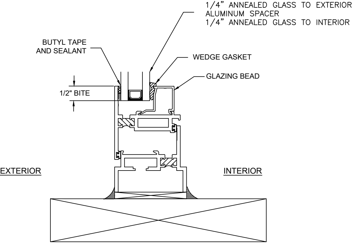
INSULATING GLASS GLAZING DETAIL
