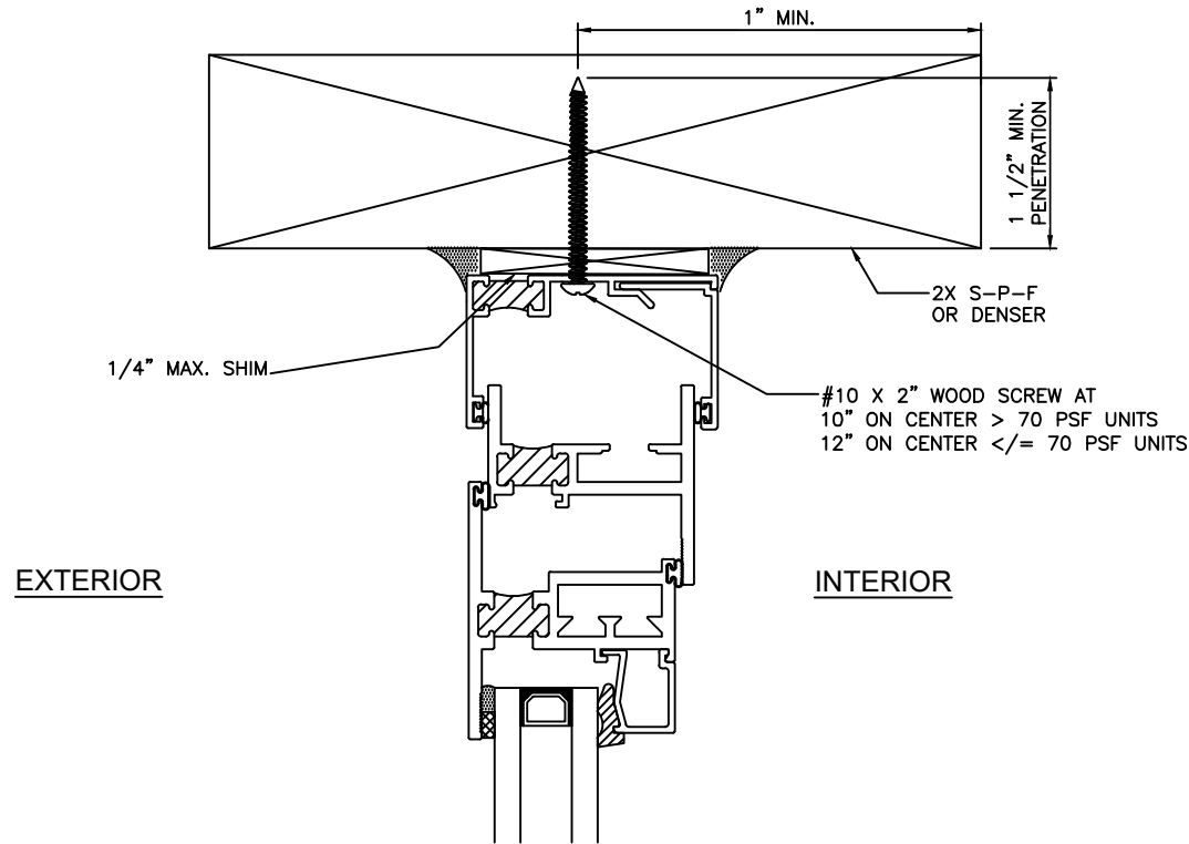
SECTION 1/1, 1/2 & 1/3 RECEPTOR TO WOOD FRAME OR BUCK SUBSILL SIMILAR
