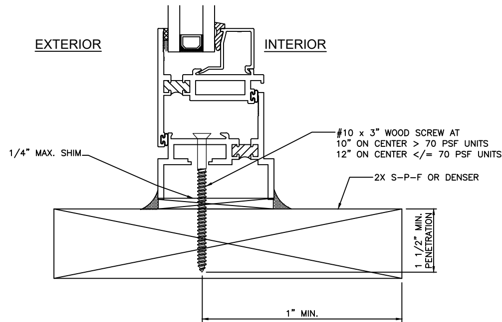
SECTION 1/1, 1/2 & 1/3 THROUGH FRAME TO WOOD FRAMING OR BUCK
