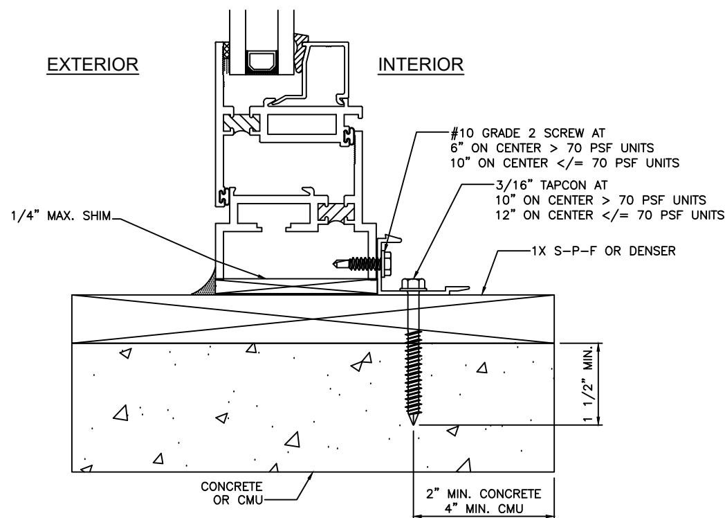
SECTION 1/1, 1/2 & 1/3 INSIDE CLIP & ANCHOR TO CONCRETE OR CMU WITH 1X BUCK STRIP
