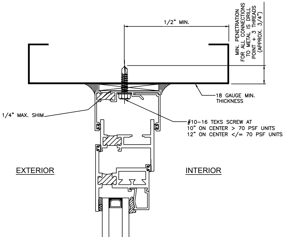
SECTION 1/1, 1/2 & 1/3 RECEPTOR TO STEEL STUD SUBSILL SIMILAR
