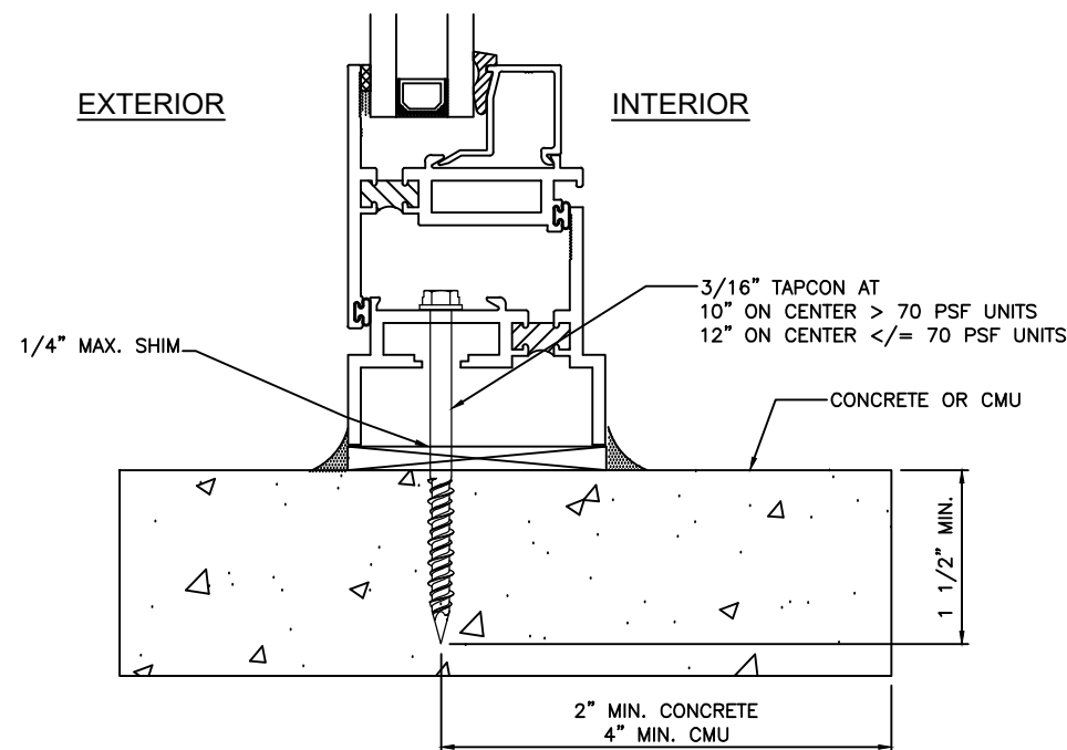
SECTION 1/1, 1/2 & 1/3 THROUGH FRAME TO CONCRETE OR CMU
